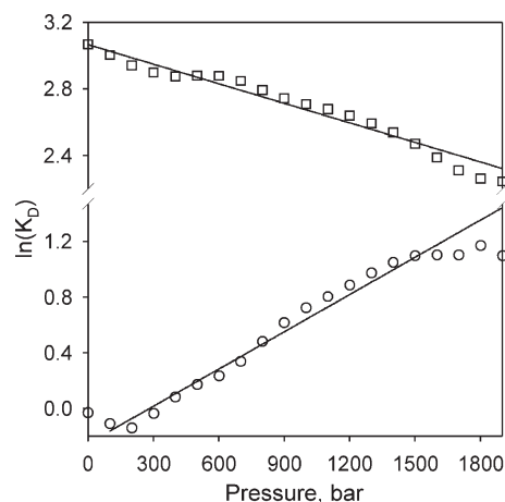
FIGURE 9: Dependencies of K_D of the P450-SS90 complexes with myristic acid (circles) and arachidonoylglycine (squares) on pressure in semilogarithmic coordinates. Lines show the linear approximations of these data sets. The respective barotropic parameters are given in Table 2.
