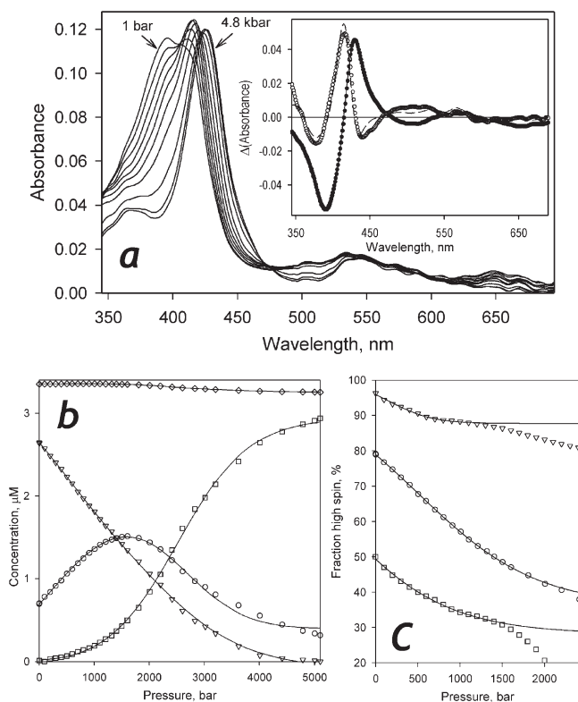
FIGURE 6: Pressure-induced transitions in P450-SS9 in the absence of substrate. Panel a represents a series of spectra recorded at pressures increasing from 1 to 2400 bar in 200 bar increments and then at 2800, 3200, 4000, and 4800 bar. The inset shows the first (closed circles) and the second (open circles) principal components found by PCA applied to this data set. Dashed lines represent the approximation of these spectra with the set of spectral standards obtained for P450-SS9 (see Supporting Information, Figure S3) Conditions: 3.5 \mu\text{M} P450-SS9 in 0.1 \text{ M} Na-Hepes buffer (pH 7.4), and 0.5 \text{ mM} EDTA, 25^\circ\text{C} . Panel b shows the corresponding changes in the concentration of the high-spin (triangles), low-spin (circles), and P420 (squares) states of P450-SS9 and the total heme protein concentration (diamonds). The pressure-induced changes in the fraction of the high-spin P450 at no substrate added (circles) and in the presence of 70 \mu\text{M} arachidonoylglycine (squares) or myristic acid (triangles) are illustrated in panel c. The full set of corresponding spin changes for substrate complexes of P450-SS9 is found in Supporting Information, Figure 4S.
