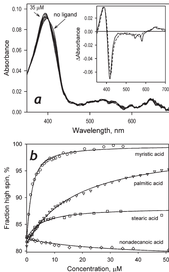
FIGURE 2: Interactions of P450-SS9 with saturated fatty acids. A series of absorbance spectra obtained in a titration of 1 μM P450-SS9 with myristic acid are shown in panel a. The inset shows the spectrum of the first principal component of the observed changes (insert) along with its approximation with the prototypic spectra of low-to-high spin transitions in P450BM-3 (dashed line). Panel b represents the titration curves of 0.8–1.2 μM P450-SS9 with a series of saturated fatty acids along with their approximations using the equation for the equilibrium of binary association.
