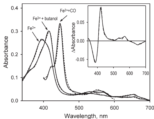
FIGURE 1: Absorbance spectra of P450-SS9. The spectra of the substrate-free ferric P450-SS9, its complex with 1-butanol, and the ferrous carbonyl complex are shown in solid lines. Dashed lines show the approximations of the spectra with combinations of the spectral standards obtained for the heme domain of P450BM-3 (22). The inset shows the butanol-induced difference spectrum (solid line) and its approximation with the prototypic spectra of high-to-low spin transitions obtained for P450BM-3 (dashed line). The spectra were recorded at 25 °C in 100 mM Na-Hepes buffer, pH 7.4, with 1 cm path length and the protein concentration of ~2 \mu M.
