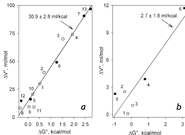
FIGURE 10: Correlation among the changes in the Gibbs free energy and the reaction volume in the spin transition of cytochromes P450. Panel a compiles the data obtained for the substrate complexes P450cam, the heme domain of P450BM3 (BMP), CYP2B4, and the “relaxed” states of CYP3A4, P450eryF, and P450-SS9. Open circles represent the data obtained with P450cam complexes with endo -borneol O -methyl ether of camphor (1), endo -borneol O -propyl ether of camphor (2), endo -borneol O -allyl ether of camphor (3), and camphor (4) (46). Closed circles show the results reported in ref 22 for the complexes of BMP with palmitic acid (5), CYP2B4 with benzphetamine (6), and P450cam with camphor (7). Open squares represent the data obtained with the complexes of P450eryF with Fluorol-7GA (26) (8) and the complexes of CYP3A4 with bromocriptine (9), testosterone (10), and 1-pyrenebutanol (11) (25). The values reported in this study for the complexes of P450-SS9 with arachidonoylglycine (12) and myristic acid (13) are shown in filled squares. The solid line represents the least-squares linear approximation of the whole data set ( \rho^2 = 0.965 ). The data characterizing the “pressure-promoted” state of P450eryF, CYP3A4, and P450-SS9 are combined in panel b. Open circles represent the data reported for the complexes of P450eryF with Fluorol-7GA (26) (1) and the complexes of CYP3A4 with testosterone (2) and 1-pyrenebutanol (3) (25). The values determined in this study for the substrate-free P450-SS9 (4) and its complexes with arachidonoylglycine (5) and myristic acid (6) are shown in filled squares. The solid line represents the least-squares linear approximation of the whole data set ( \rho^2 = 0.834 ).
