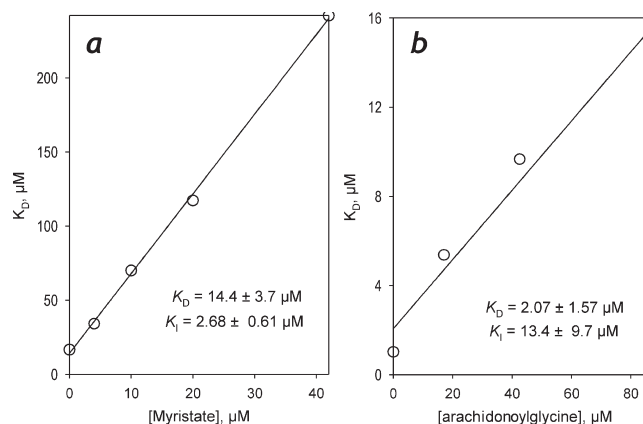
FIGURE 5: Competition of myristic acid and arachidonoylglycine for the interactions with P450-SS9. Mutual effects of myristic acid and arachidonoylglycine on the effective constant of dissociation of the P450-SS9 complex with their counterparts are shown in panels a and b, respectively. Solid lines show the linear approximations of the data with the parameters ( K_I for the competitor and K_D for the titrant) shown.
