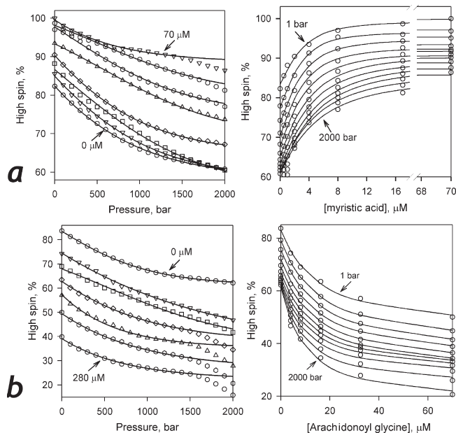
FIGURE 7: Effect of hydrostatic pressure on the spin state of P450-SS9 in solution at increasing concentrations of myristic acid (a) and arachidonoylglycine (b). The plots shown on the left of each panel represent the content of the high-spin state as a function of pressure at various concentrations of substrates (0.5, 1.0, 2.0, 4.0, 8.0, 16.0, 32.0, and 70.0 \mu\text{M} myristic acid and 4.0, 8.0, 16.0, 32.0, 70.0, and 280.0 \mu\text{M} arachidonoylglycine for panels A and B, respectively). The plots shown on the right represent the same data set shown as the changes in the high-spin content with increasing substrate concentration at a series of pressures increasing from 1 to 2000 bar in 200 bar increments. Solid lines show the results of fitting of the titration curves to the equation for the equilibrium of binary association.
