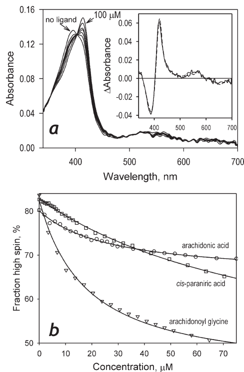
FIGURE 4: Interactions of P450-SS9 with unsaturated fatty acids and arachidonoylglycine. A series of absorbance spectra obtained in a titration of 1.8 \mu\text{M} P450-SS9 with arachidonoylglycine is shown in panel a. The inset shows the spectrum of the first principal component of the observed changes (insert) along with its approximation with the prototypic spectra of high-to-low spin transitions in P450BM-3 (dashed line). Panel b represents the titration curves of 0.8–1.8 \mu\text{M} P450-SS9 with a series of saturated fatty acids along with their approximations using the equation for the equilibrium of binary association.
