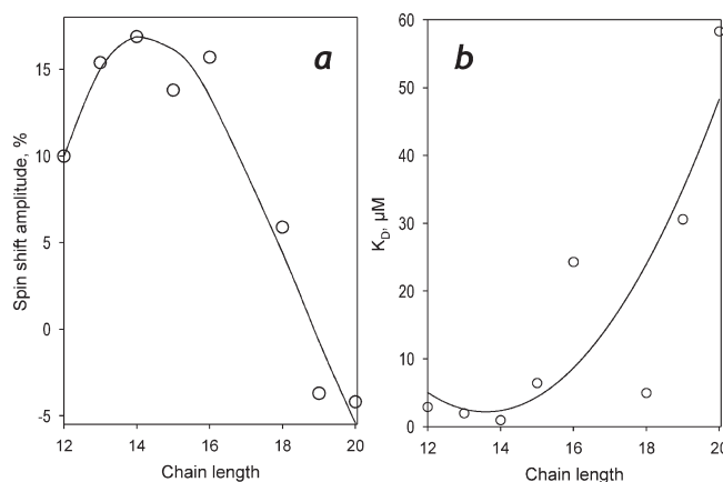
FIGURE 3: The amplitude of the spin shift (a) and the dissociation constant (b) characterizing the interactions of P450-SS9 shown as a function of the length of the alkyl chain. The solid lines represent the approximation of the data sets with a third-order polynomial. These approximations have no interpretative meaning and are shown only to illustrate the general trend of the dependencies.
